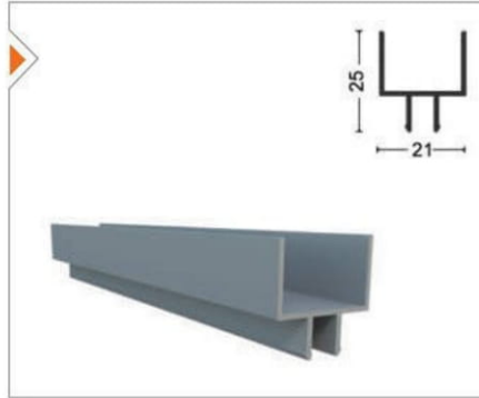
YNSRM-1008 Isıcam Adaptörü Converter Adapter
