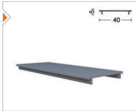
GYTN-1511 Yan Dikme Kapağı Side Cover Profile
