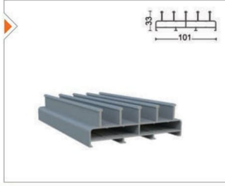
SRM-1002 Eşikli Alt Kasa Profili With Threshold - Lower Frame Profile
