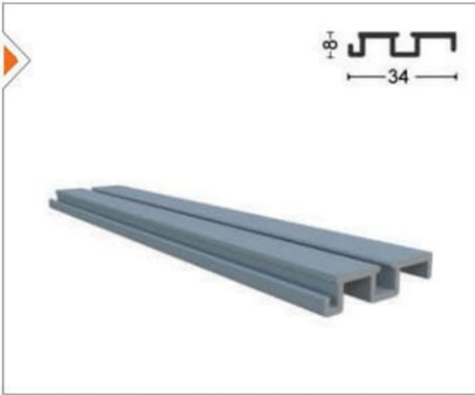
YNSRM-1004 Eşiksiz Ek Profil Additional Profile (Without Threshold)
