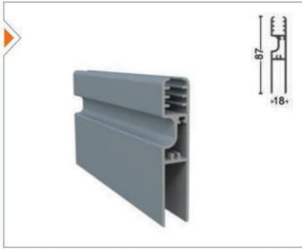
SRM-1004 Baza 8 mm Profili Aluminum Glass Profile (8 mm)
