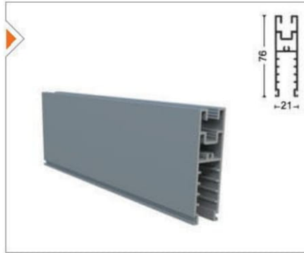
YNSRM-1005 Baza Profili Aluminum Glass Profile
