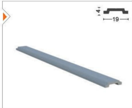
ISICM31-1013 Tij Profili Ağrlık/Weight Push Rod Profile 0.123 kg/m
