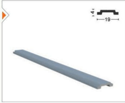
ISICM31-1013 Tij Profili Push Rod Profile
