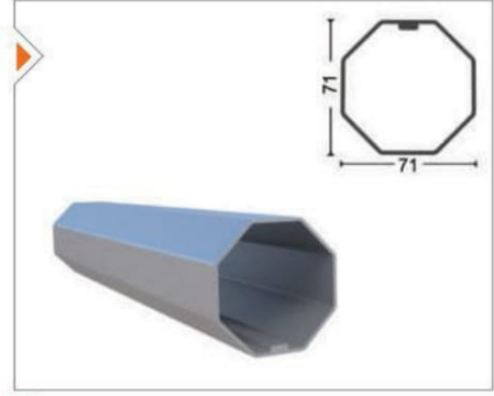
GYTN-1503 70'lik Sekizgen Boru Octagonal Aluminum Tubing
