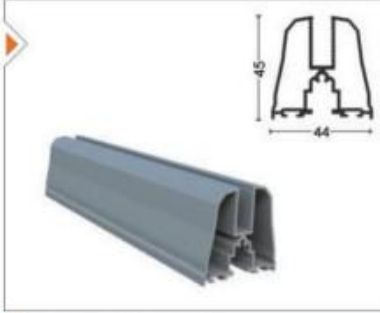
PRGLD-1002 Baza Profili Aluminum Glass Profile
