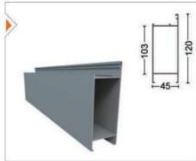
AD-1010 Aldoks Etek Profil Aldox Bottom Rail Profile
