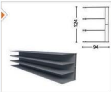
GYTN-1510 Yan Dikme Profili Aluminum Side Profile
