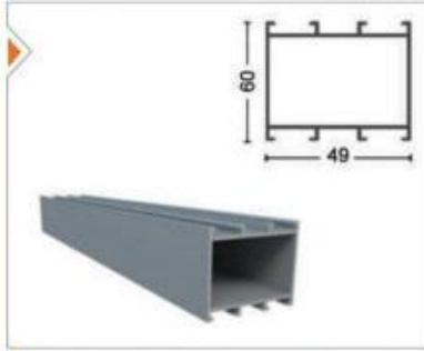
C60-1001 C-60 Kasa Profili C-60 Frame Profile
