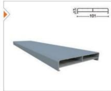
SRM-1006 Yan Dikme Profili Aluminum Side Profile
