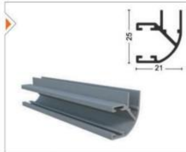
ALMFTL-1004 90° Fitol Aluminum 90° Seal
