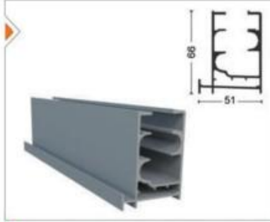
GLDPLS-1002 Oluklu Kasa Profili Dropper Frame Profile
