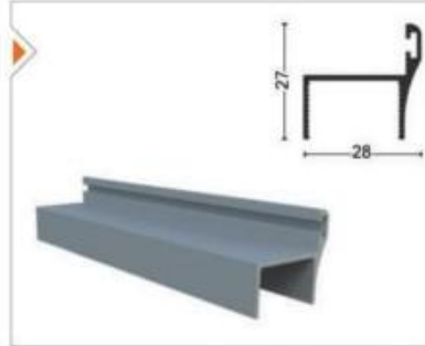
ISiCM21-1004 Küçük h Fıtil Small "h" Aluminum Seal
