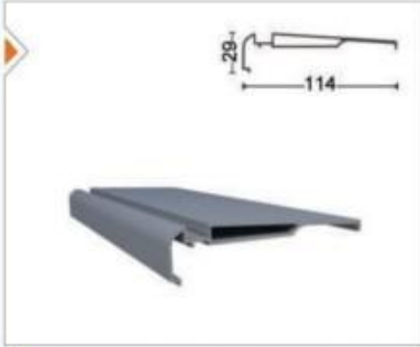
GYTN-1504 Küpeste Profili Railing Profile
