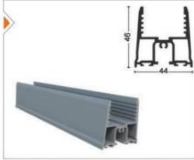
ISICM31-1001 Baza Profili Aluminum Glass Profile
