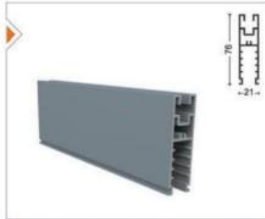
YNSRM-1005 Baza Profili Aluminum Glass Profile
