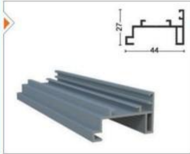
ISICM31-1012 Kollu Fitol Karşıklı Contalı Exp. Handle Opposite Alm. Seal (With Pvc Seal)
