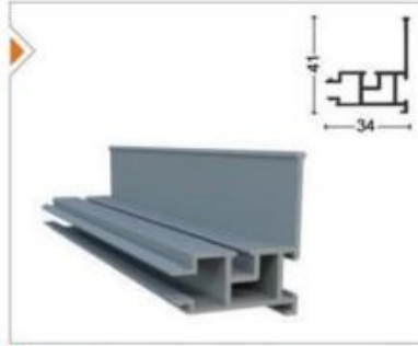
YNSRM-1002 Eğikli Ek Profil Additional Profile (With Threshold)
