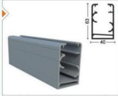
GLD-1001 Kasa Profili Frame Profile
