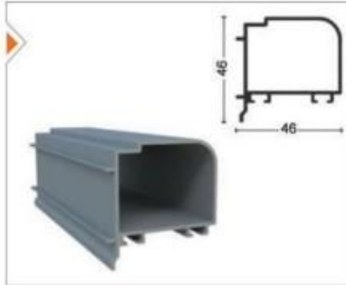
ISICM31-1014 90° Adapter Aluminum 90° Seal
