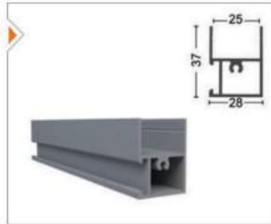
GYTN-1509 Baza İsicam Profili Aluminum Double Glass Profile
