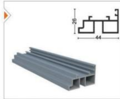
PRGLD-1006 Kollu Fitol Karşılığı Contalı Esp. Handle Opposite Alm. Seal (With Pvc Seal)
