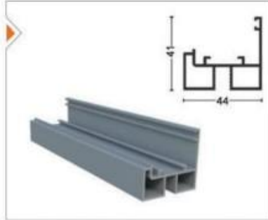
PRGLD-1005 Kollu Fıtlı Contalı Esp. Handle Alm. Seal (With Pvc Seal)
