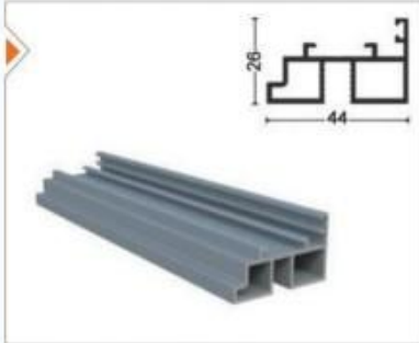
PRGLD-1006 Kollu Fıtlı Karşılığı Contalı Esp. Handle Opposite Alm. Seal (With Pvc Seal)
