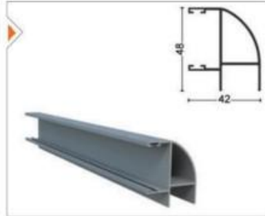
ISiCM21-1007 90° Fıtil Aluminum 90° Seal
