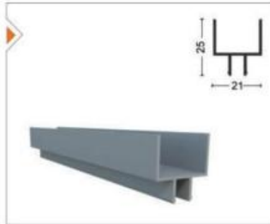
YNSRM-1008 Isıcam Adaptörü Converter Adapter
