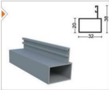
GLD-1004 Yan Kasa Profili Aluminum Side Profile
