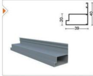
ISiCM21-1002 Yan Kasa Profili Aluminum Side Profile
