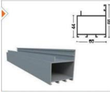
C60-1002 C-60 Kanat Profili C-60 Sash Profile
