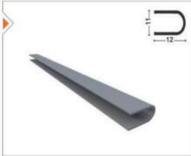
ALMFTL-1005 D Fitol Aluminum 'D' Seal
