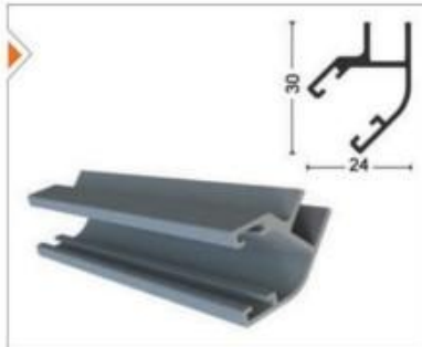
ALMFTL-1003 135° Fitol Aluminum 135° Seal
