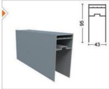
GLD-1005 Perdelik Ayar Profili Aluminum Curtain Profile
