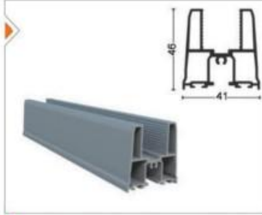
ISiCM21-1001 Baza Profili Aluminum Glass Profile
