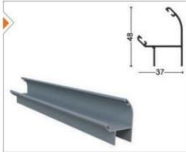
ISiCM21-1006 135° Fıtil Aluminum 135° Seal
