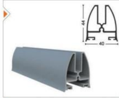
GLDPLS-1003 Baza Profili Aluminum Glass Profile
