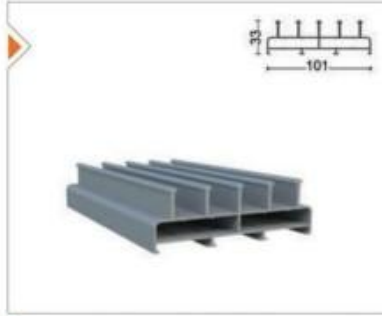
SRM-1002 Eğikli Alt Kasa Profili With Threshold - Lower Frame Profile
