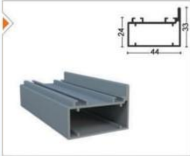
ISICM31-1009 Yan Kasa Profili Aluminum Side Profile (With Pvc Seal)
