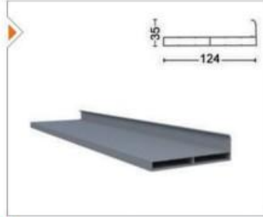
GYTN-1506 Alt Kasa Profili Lower Frame Profile
