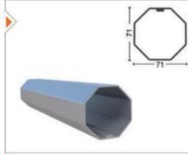
GYTN-1503 70'lik Sekizgen Boru Octagonal Aluminum Tubing
