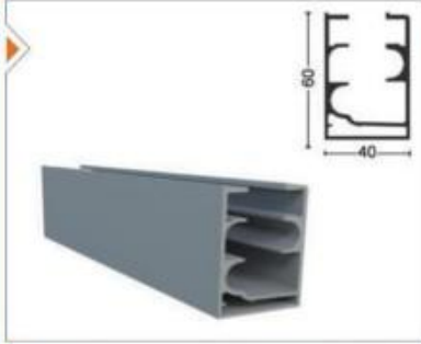
GLDPLS-1001 Kasa Profili Frame Profile
