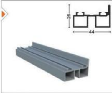
PRGLD-1004 Küçük h Fıtlı Contalı Aluminum Small h Seal (With Pvc Seal)
