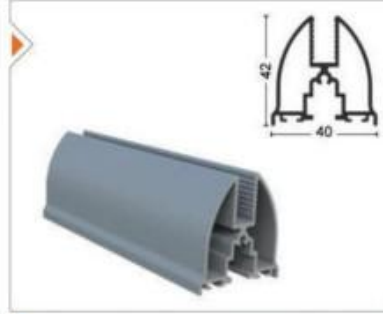
GLD-1003 Baza Profili Aluminum Glass Profile
