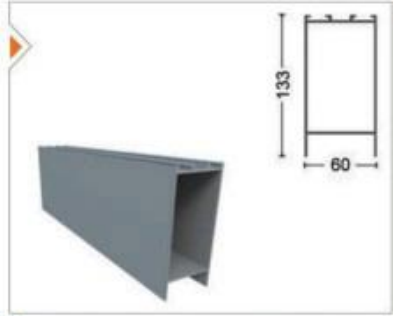
C60-1003 C-60 Etek Profili C-60 Bottom Rail Profile
