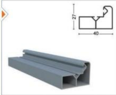
GLDPLS-1004 Yan Kasa Aluminum Side Profile
